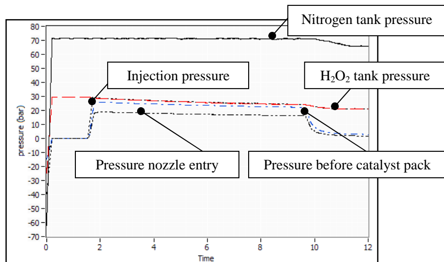
Figure 7 : Typical result by using 1.367mm diameter injector which is not achieve 0.7MPa pressure drop.
