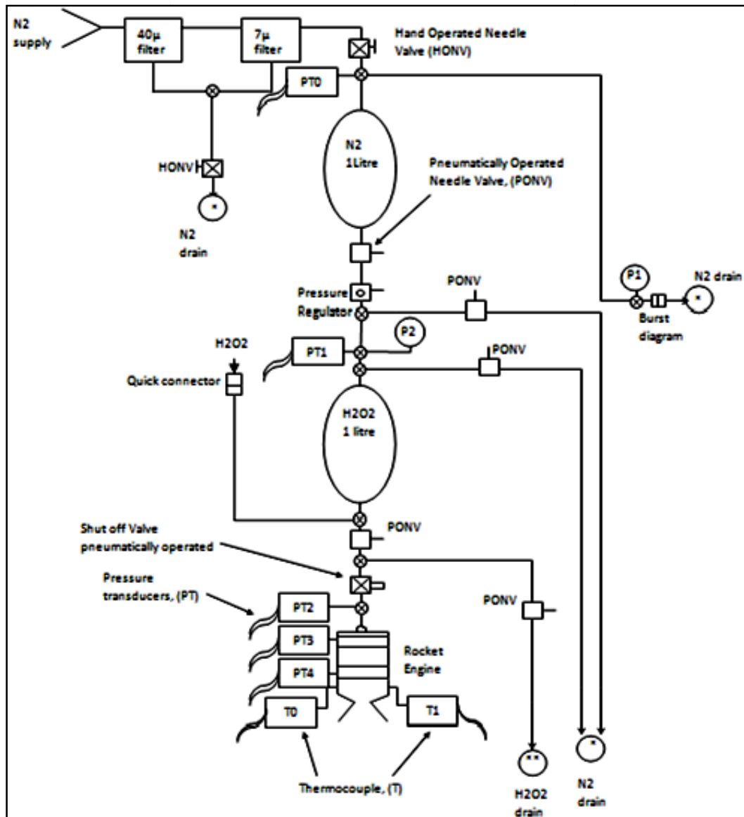
Figure 6 : Line diagram of hydrogen peroxide rocket thruster facility.
