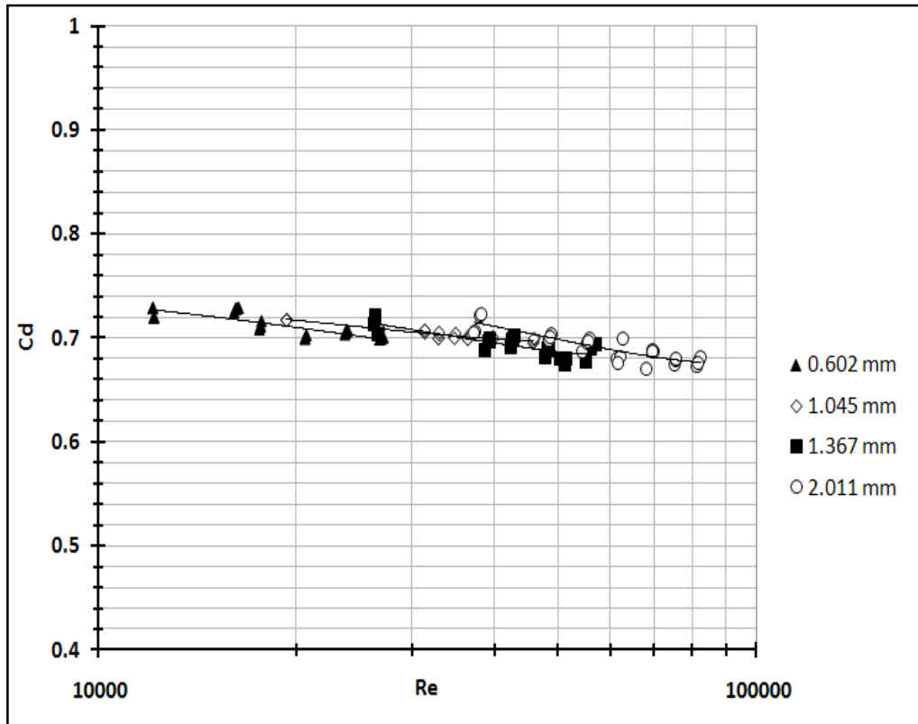
Figure 5 : Discharge coefficient for four different diameter injectors.
