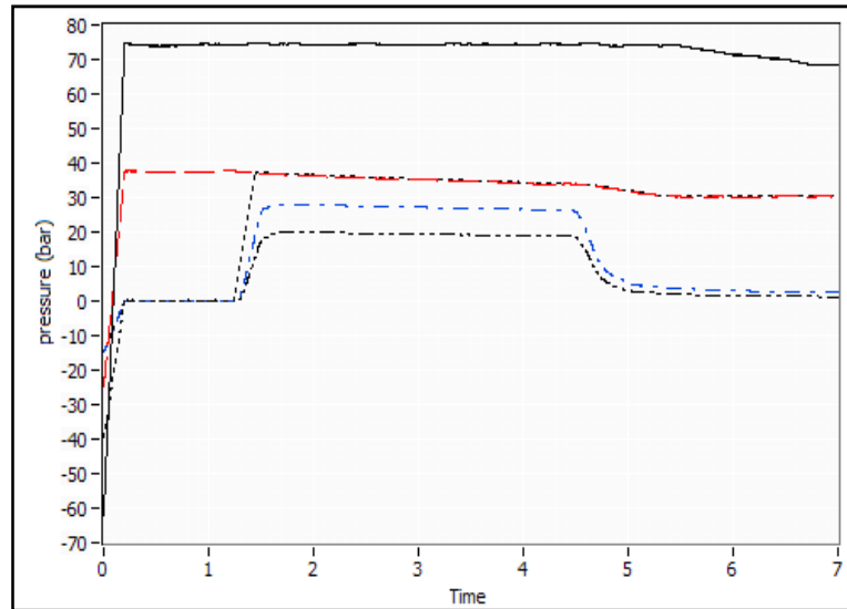
Figure 8 : Successful result by using 1.045mm diameter injector which is achieve 0.7MPa pressure drop.
