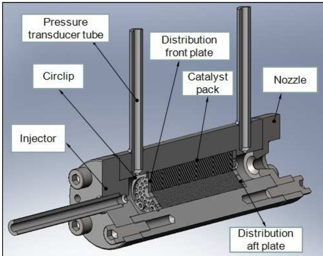
Figure 2 : Quarter section view of 50 N hydrogen peroxide thruster.
