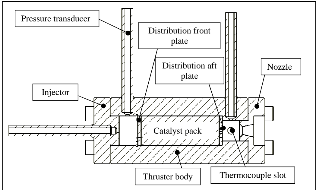
Figure 1: 50N hydrogen peroxide rocket thruster.
